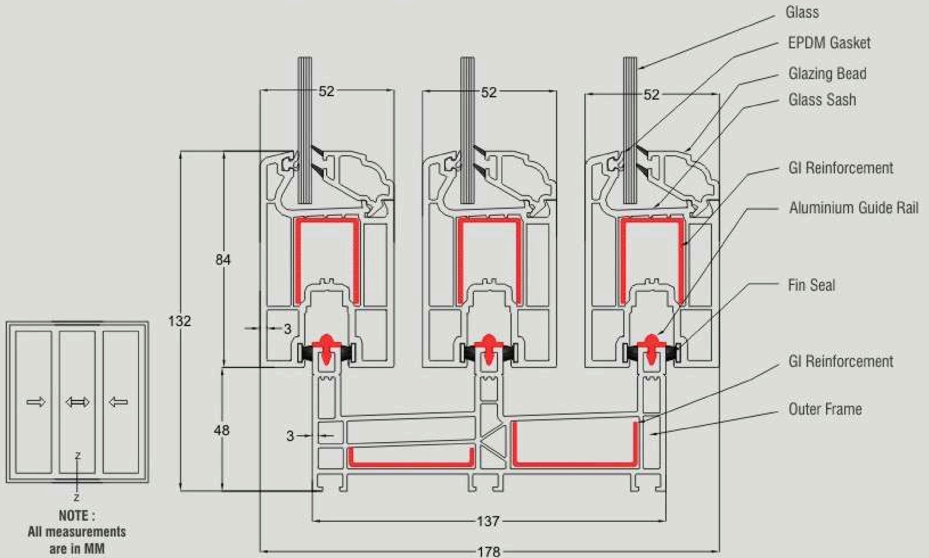
Cross Section of Sliding Door (3track 3panel) Without Mesh
